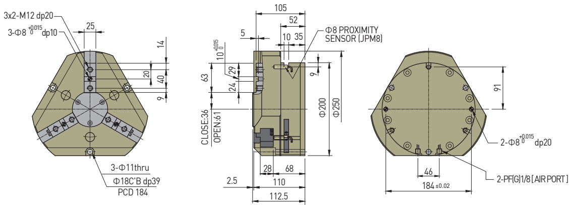
■ BP (Bottom Port) DIMENSION
