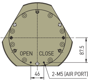
■ BP (Bottom Port) DIMENSION
