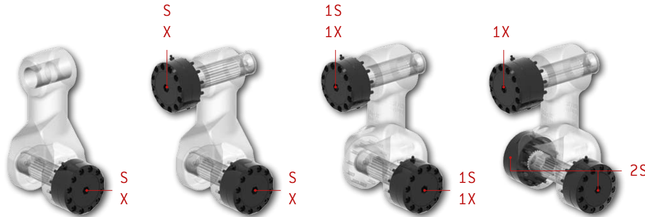
BRAKE STRUCTURE FOR R-LINKS
