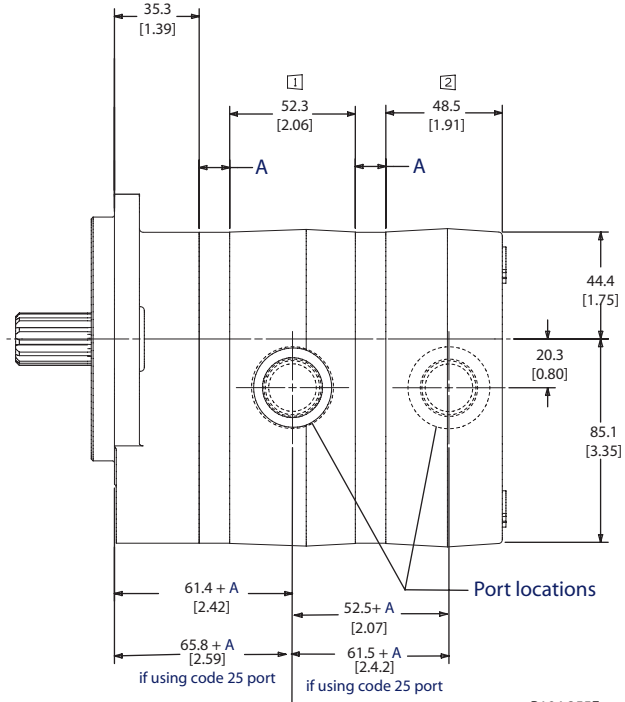
Multiple section pump dimensions
