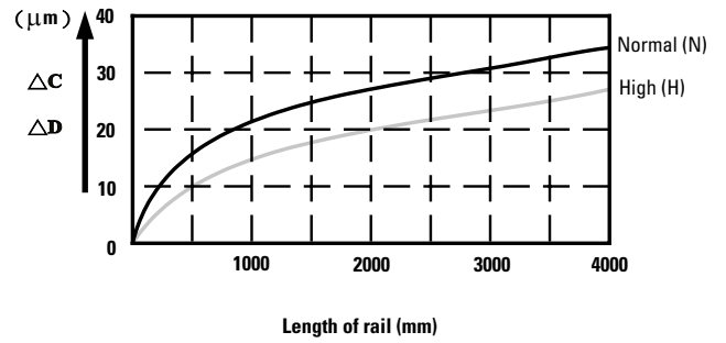
Fig. 1-1 400 Series rail length and running parallelism
