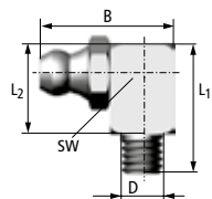
530LN90 Hydraulic-type lubricating nipple, 90° angle
